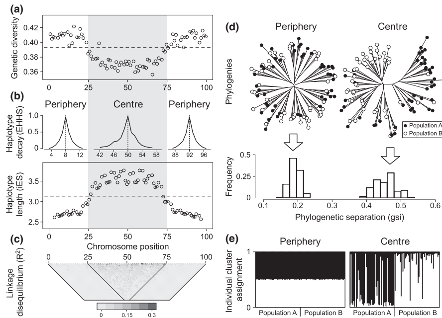
FIGURE 7 Consequences of heterogeneity in crossover rate beyond CCBD. (a) Divergence with gene flow and a relatively reduced crossover rate in the chromosome centre leads to lower genetic diversity in the chromosome centre (shaded in grey) than in the peripheries within a population. The dots are means over both populations and 100 simulation replicates, and the dashed horizontal line indicates the mean across the entire chromosome. (b) The rate of haplotype decay within a population is lower around loci in the chromosome centre than around peripheral loci, as shown for two exemplary loci from the chromosome periphery (positions 8 and 92) and a locus from the chromosome centre (position 50). The lower panel displays a locus-specific haplotype length metric along the entire chromosome (dots are means across both populations from 25 replicates). (c) As a consequence of longer haplotype tracts, loci in the chromosome centre also exhibit extended linkage disequilibrium within a population. (d) With a heterogeneous crossover rate, loci from the chromosome centre exhibit stronger phylogenetic separation between populations than loci from the periphery. The upper panel shows neighbour-joining trees based on subsamples from both populations generated in a single simulation. The lower panel describes the strength of phylogenetic separation expressed by the genealogical sorting index (gsi) based on central versus peripheral loci across 100 replicate simulations. (e) Diverging populations also appear genetically more distinct when applying the STRUCTURE clustering algorithm to central versus peripheral loci. Individual assignment probabilities to each of two genetic clusters (black and white) are visualized by vertical bars. Data are from a single simulation replicate. With default parameters, loci from the centre indicate two distinct populations whereas peripheral loci indicate a single homogeneous cluster. (a–e) are all based on the standard model and consider the NL only
